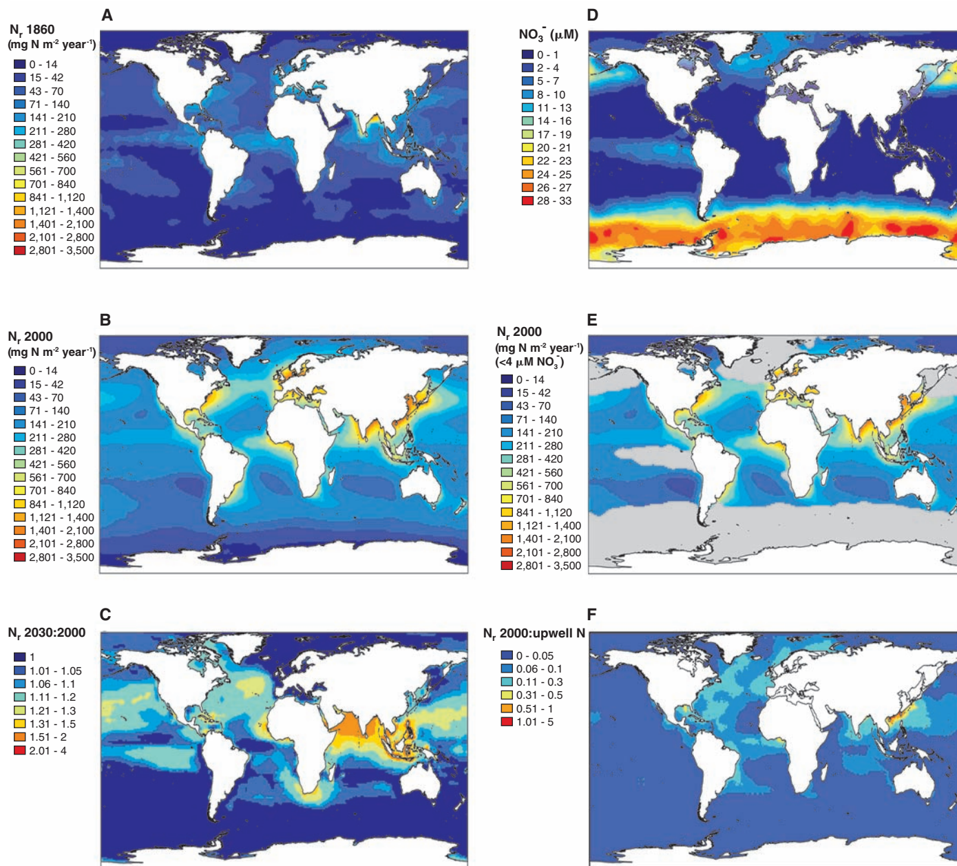
Fig. 1. (A) Total atmospheric reactive nitrogen ( \text{N}_r ) deposition in \text{mg m}^{-2} \text{ year}^{-1} [ \text{NH}_x and \text{NO}_y are derived from (3), with the addition of 30% of the total nitrogen as organic nitrogen]. Total atmospheric \text{N}_r deposition in 1860 was \sim 20 \text{ Tg N year}^{-1} , AAN was \sim 5.7 \text{ Tg N year}^{-1} . (B) Total atmospheric reactive nitrogen ( \text{N}_r ) deposition in 2000 in \text{mg m}^{-2} \text{ year}^{-1} [derived from (21) with the addition of 30% of the total nitrogen as organic nitrogen]. Total atmospheric \text{N}_r deposition in 2000 was \sim 67 \text{ Tg N year}^{-1} , AAN was \sim 54 \text{ Tg N year}^{-1} . (C) Ratio of the projected flux of \text{N}_r to the ocean in 2030 to
